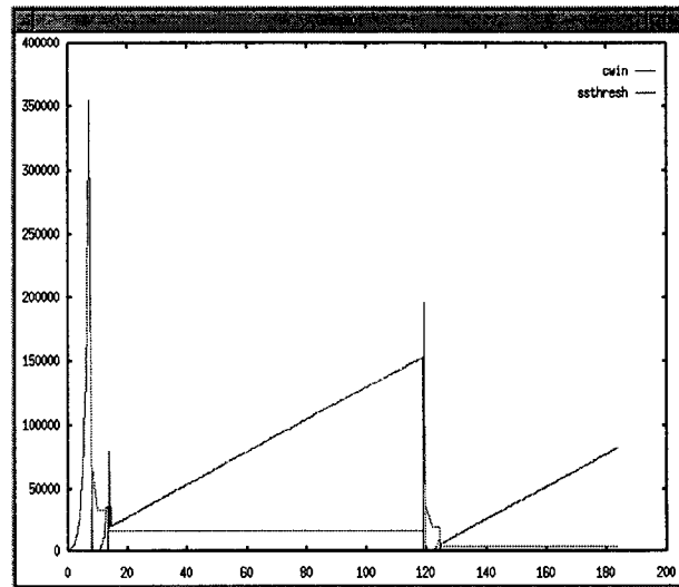
Figure 29: Effect of high initial setting of ssthresh on cwin expansion over long-delay with large window – cwnd collapses to a very low value after 8s because of a slow-start phase that lasts too long
