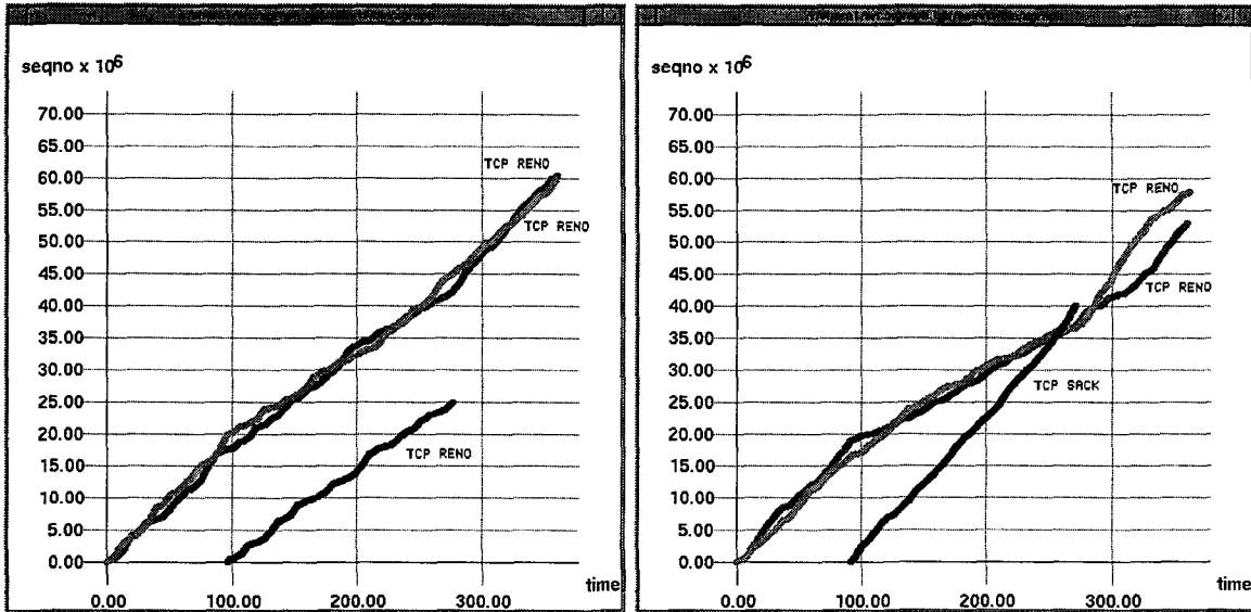
Figure 32: Second example (link delay=50ms, bandwidth=10MB/s)
