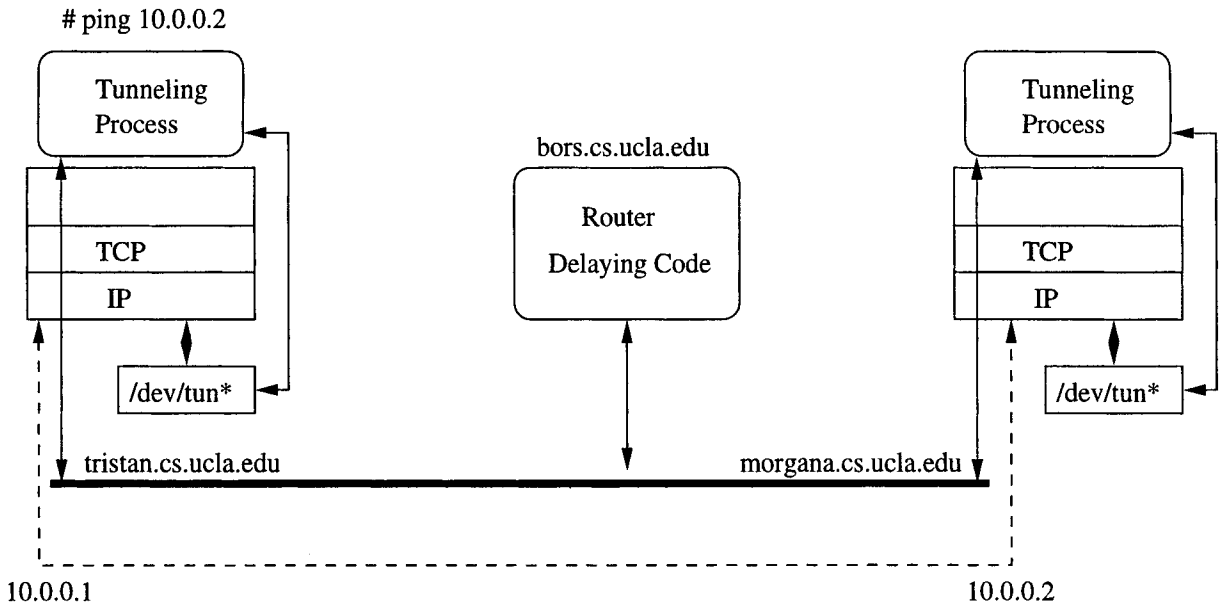
Figure 1: Testbed – Tunneling to emulate delay
